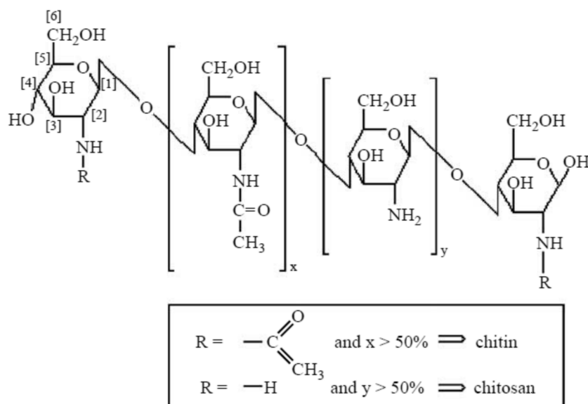
Fig. 1. Schematic representation of chitin and chitosan depicting the co-polymer character of biopolymers (Khor 2001).
