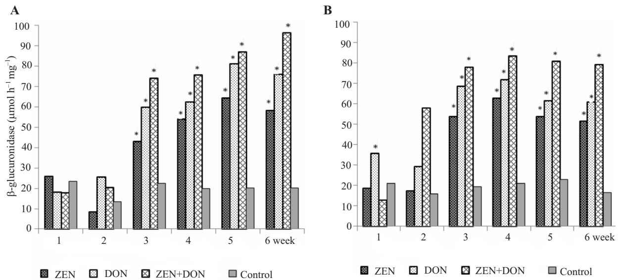
Fig. 2. Activity of \beta -glucuronidase in the proximal (A) and distal colon (B) of gilts after experimentally induced Fusarium mycotoxigenesis. Results significantly different (*) from the control in a given week of experiment, ANOVA ( P < 0.05 ).
