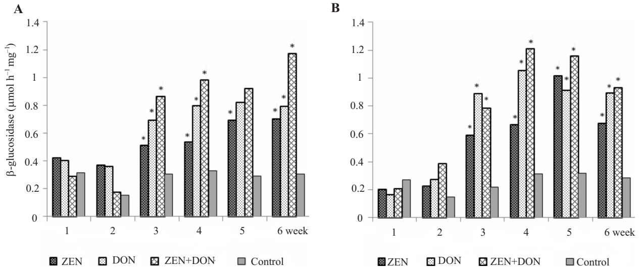
Fig. 1. Activity of \beta -glucosidase in the proximal (A) and distal colon (B) of gilts after experimentally induced Fusarium mycotoxigenesis. Results significantly different (*) from the control in a given week of experiment, ANOVA ( P < 0.05 ).
